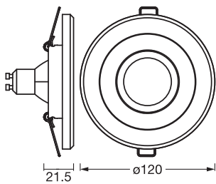
DECOR SPOT WOOD 4.5W GU10
