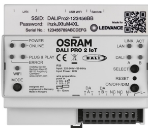
OSRAM DALI PRO 2 IoT LDVV EAN: 4052899627079
